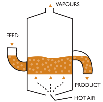
FLUIDISED BED DRYER
