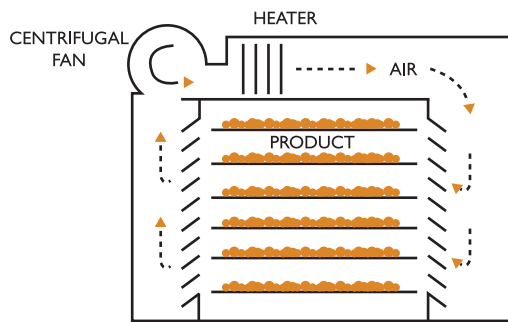
TRAY DRYER
